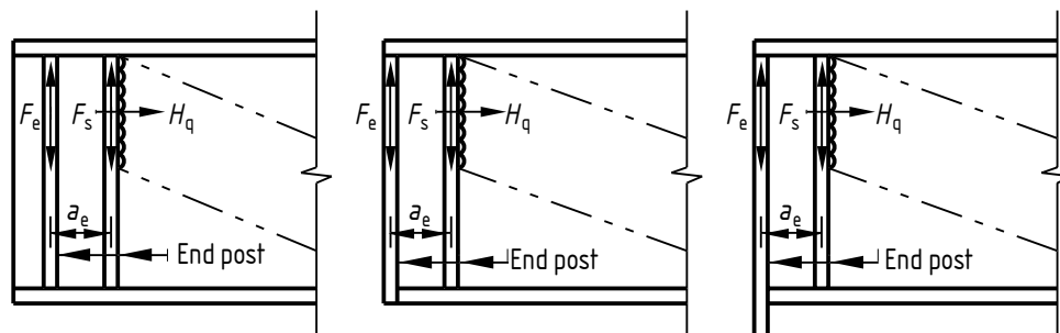
Figure H.3 — Twin stiffener end posts
